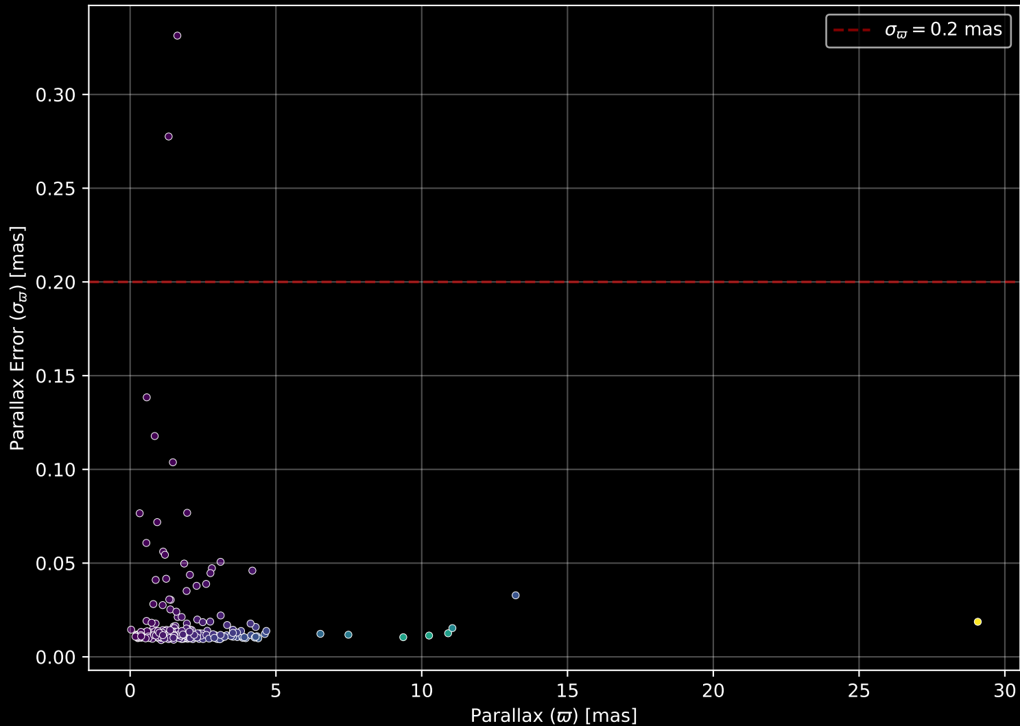
GALAH DR4 Field: [7006] Parallax Quality (n= 299)
