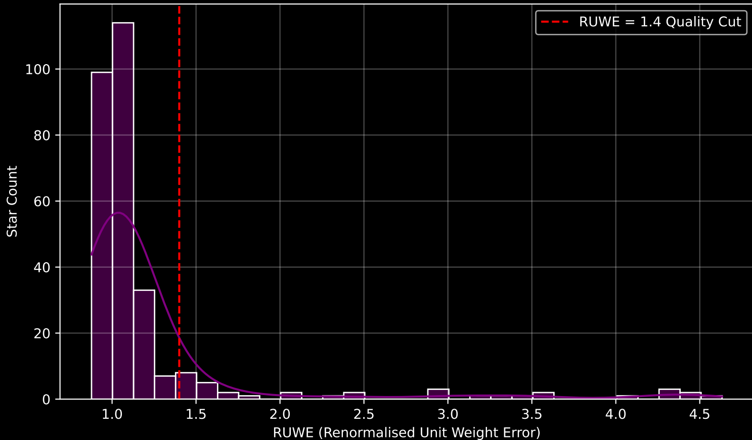
GALAH DR4 Field [7006] RUWE Distribution (n= 289)
