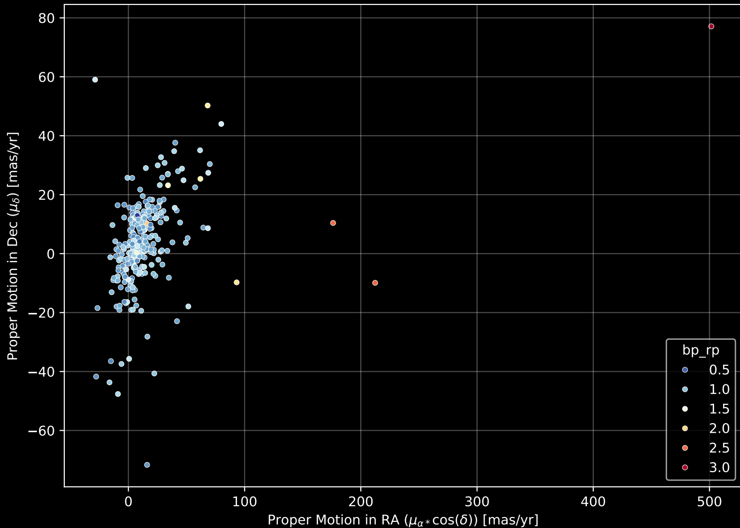
GALAH DR4 Field: [7006] Proper Motion Diagram (n= 299)
