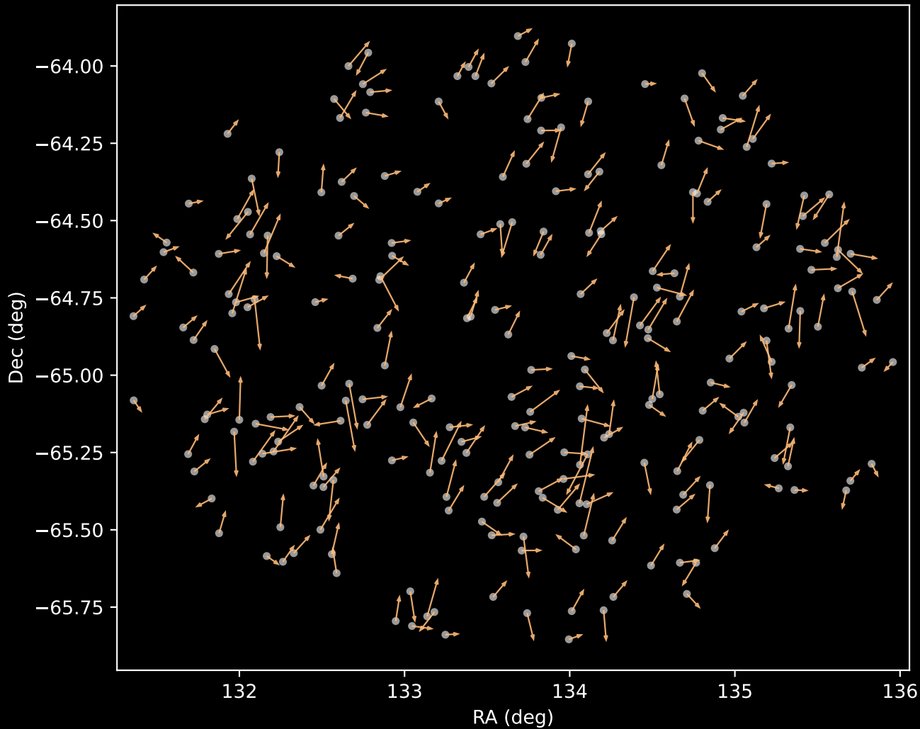
GALAH DR4 Cluster 3 Proper Motion Vectors (n=242)
