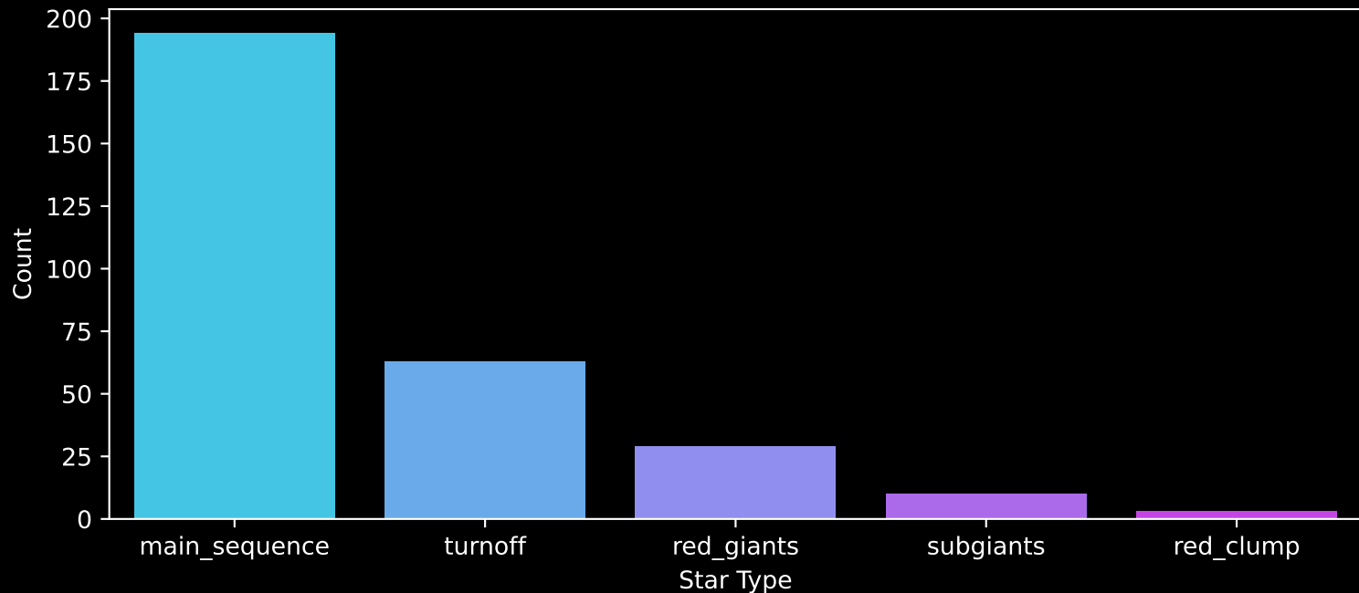
GALAH DR4 Field: [7006] Count plot of Star Type
